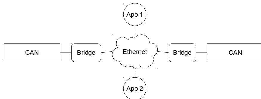
Figure 2: Setup with multiple CAN buses
